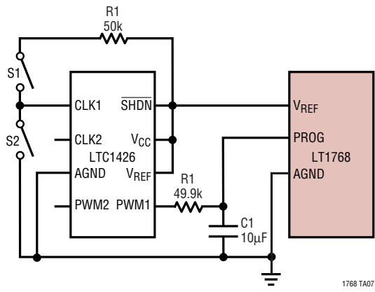
Pushbutton Intensity Control
